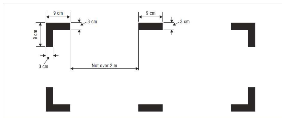
MARKING OF BREAK-IN POINTS (see 4.2.4.)
